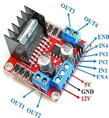
Fig 2.Motor Driver Module
