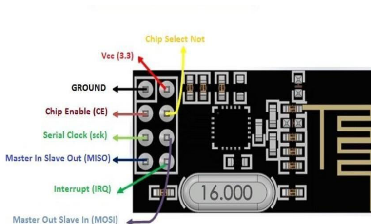
Fig.6. NRF24L01 Pin Diagram
