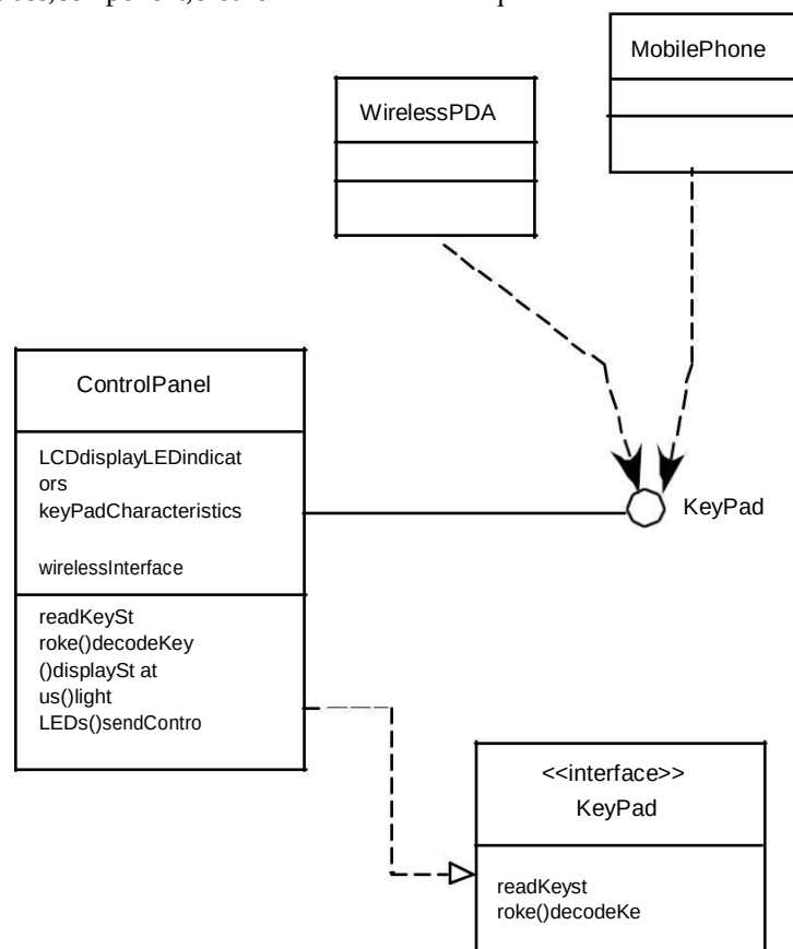
Figure 9.6 UML interface representation for Control Panel
